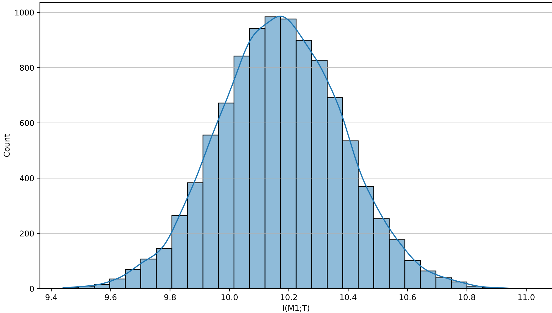
I(M1;T) distribution
