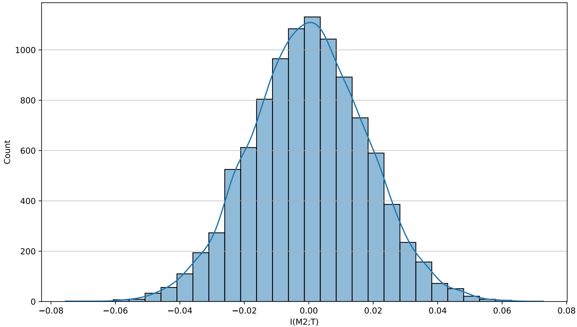
I(M2;T) distribution
