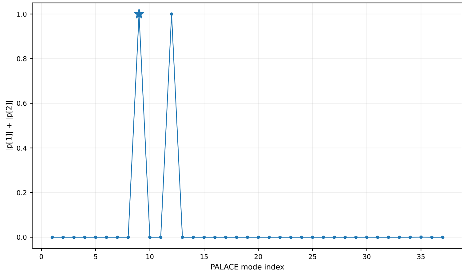
Q1 junction participation across eigenmodes
