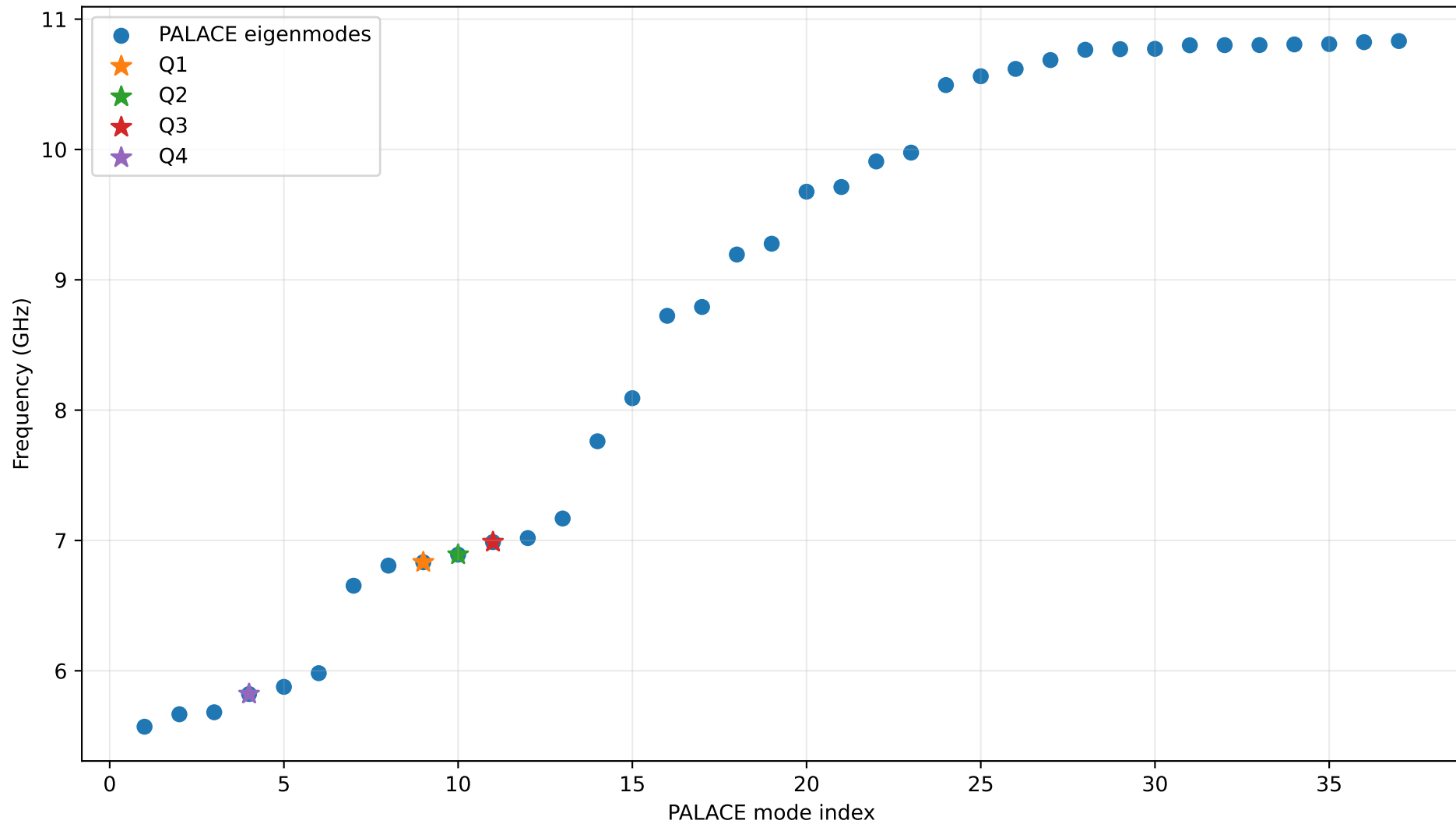
Full-chip PALACE eigenmode spectrum
