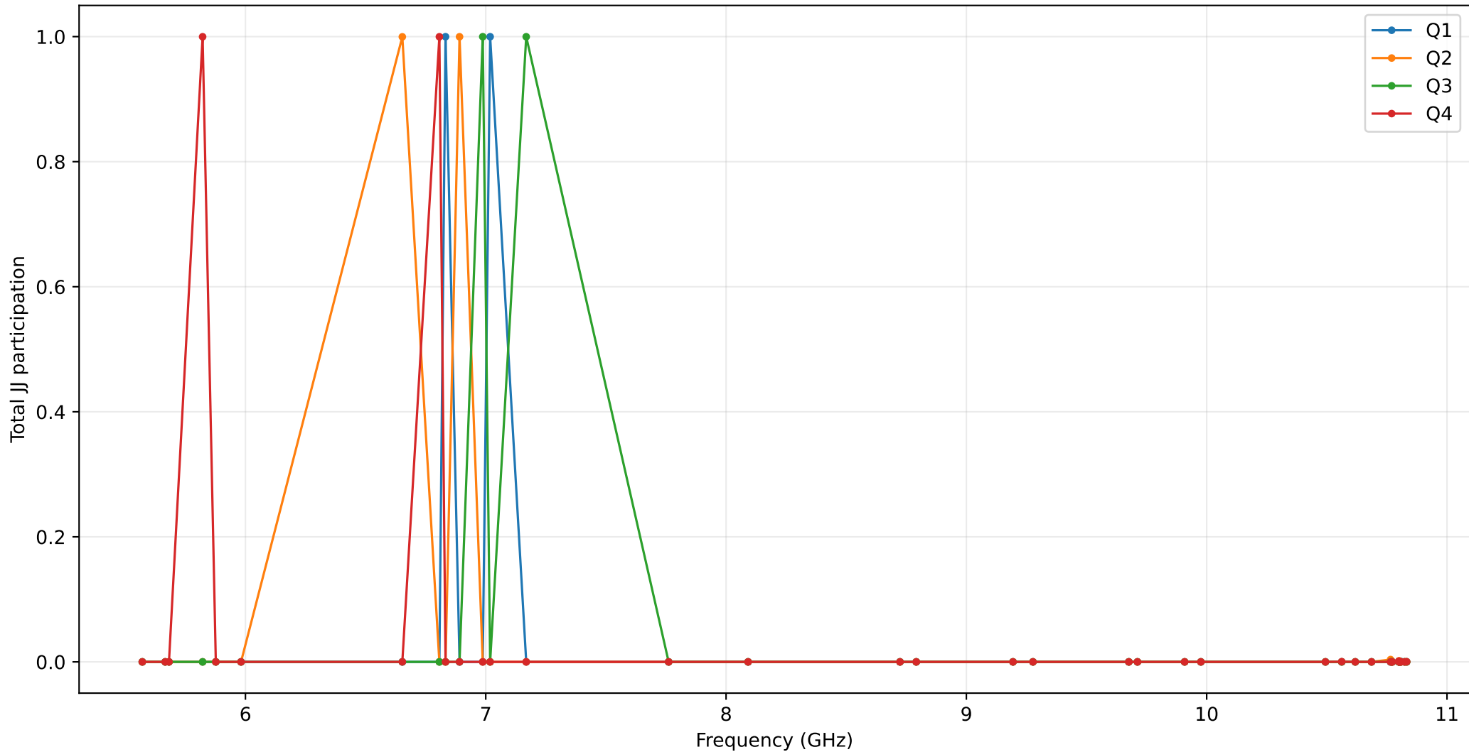
Qubit-sector participation across the full PALACE spectrum
