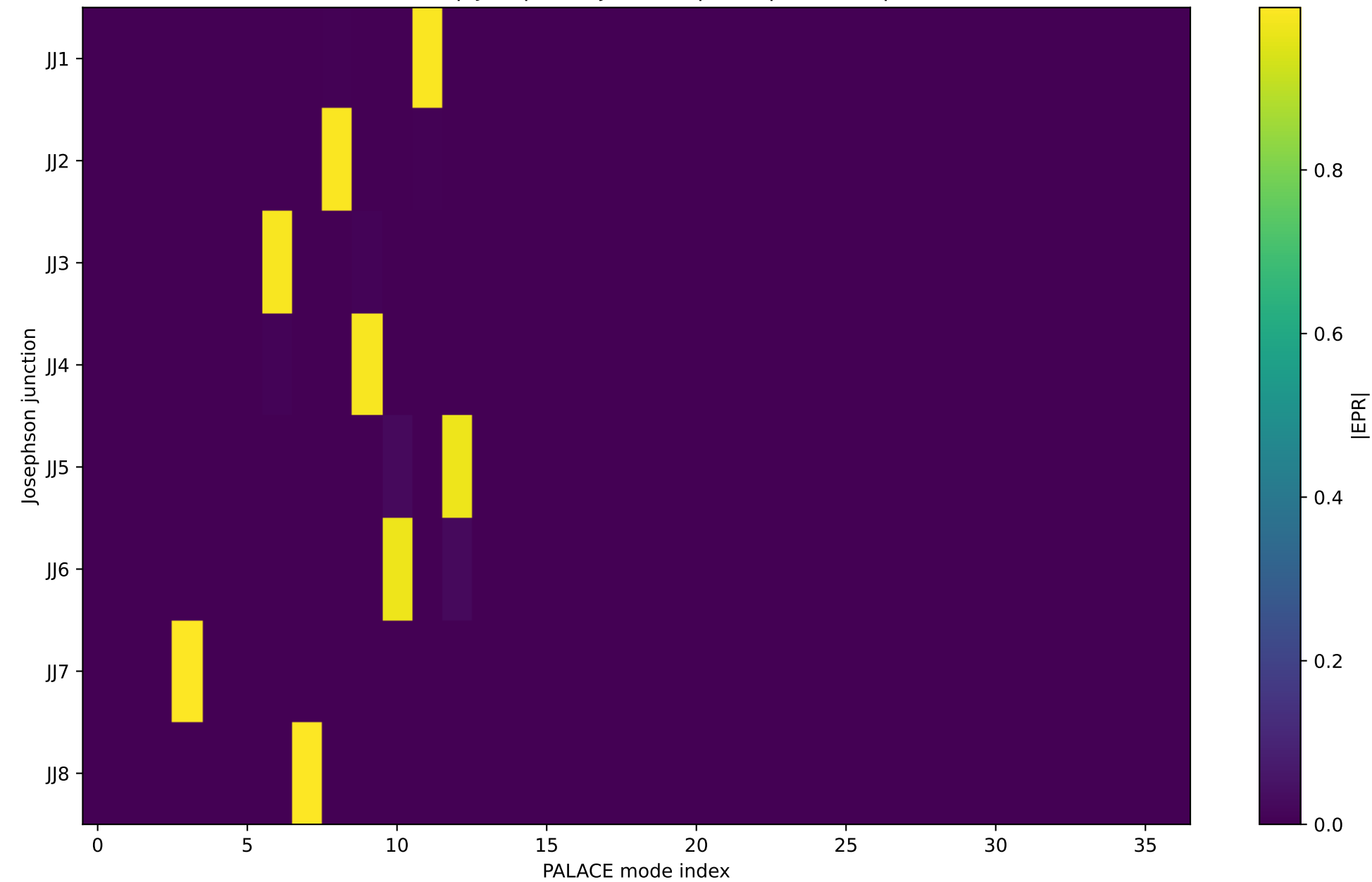
Full-chip Josephson-junction participation map
