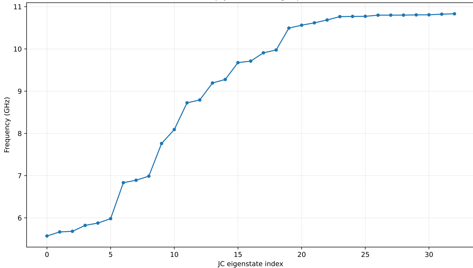
Multimode Jaynes-Cummings spectrum
