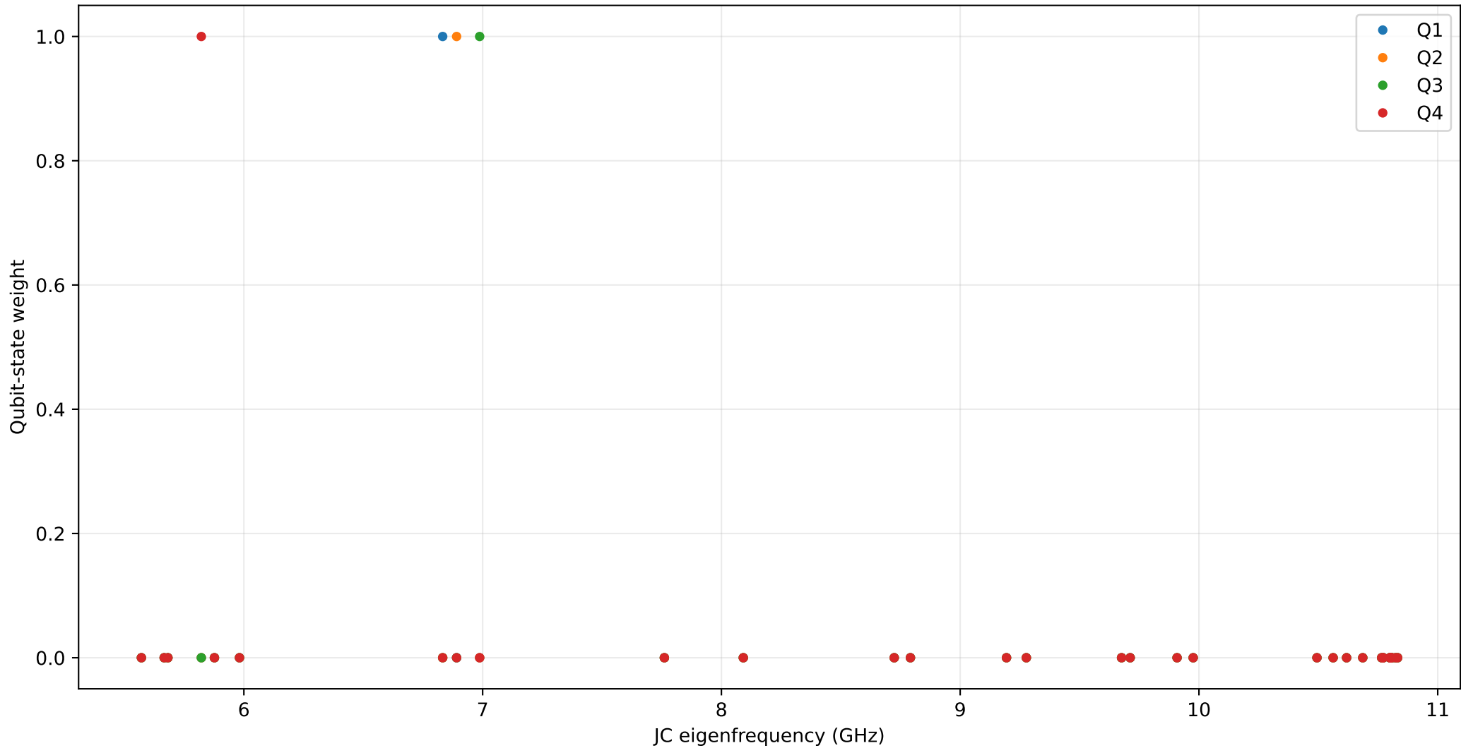
Qubit character of multimode JC eigenstates
