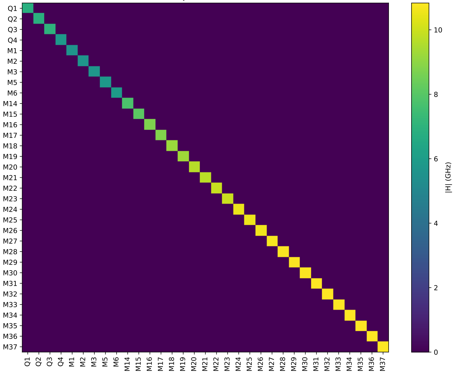
Multimode JC Hamiltonian matrix
