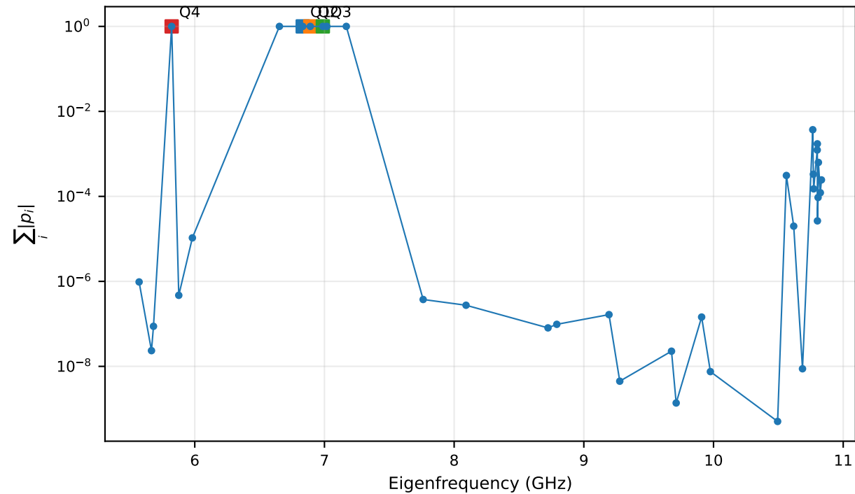
PALACE eigenmode spectrum and JJ-port localization
