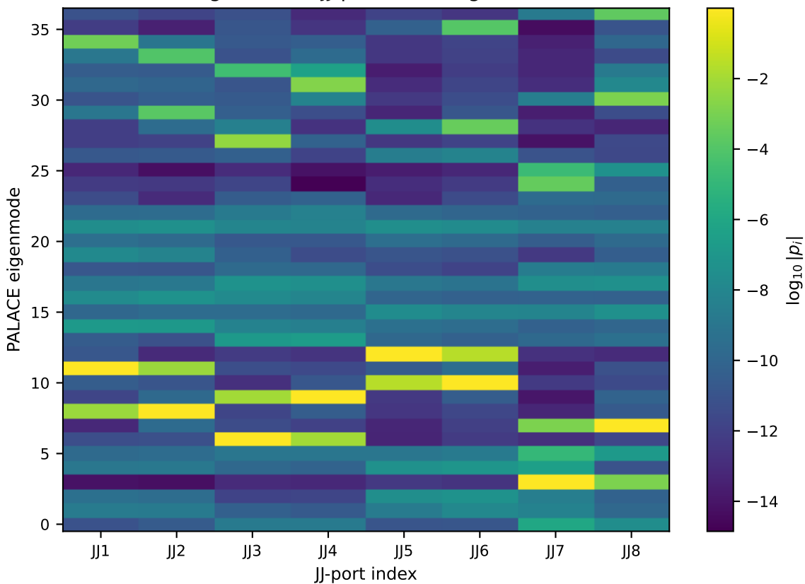
Magnitude of JJ-port EPR diagnostics
