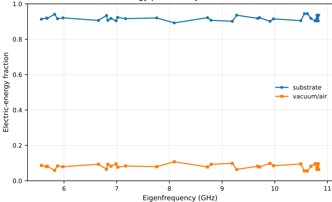
Electric-energy partition by dielectric domain
