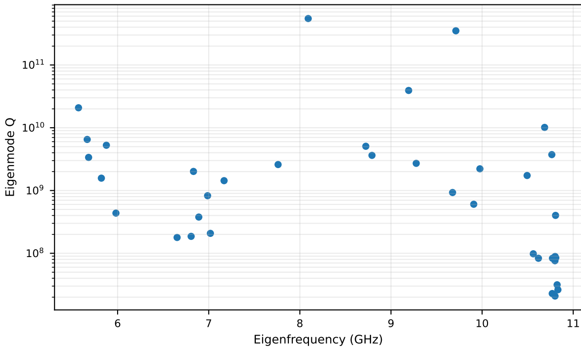
PALACE eigenmode quality factors
