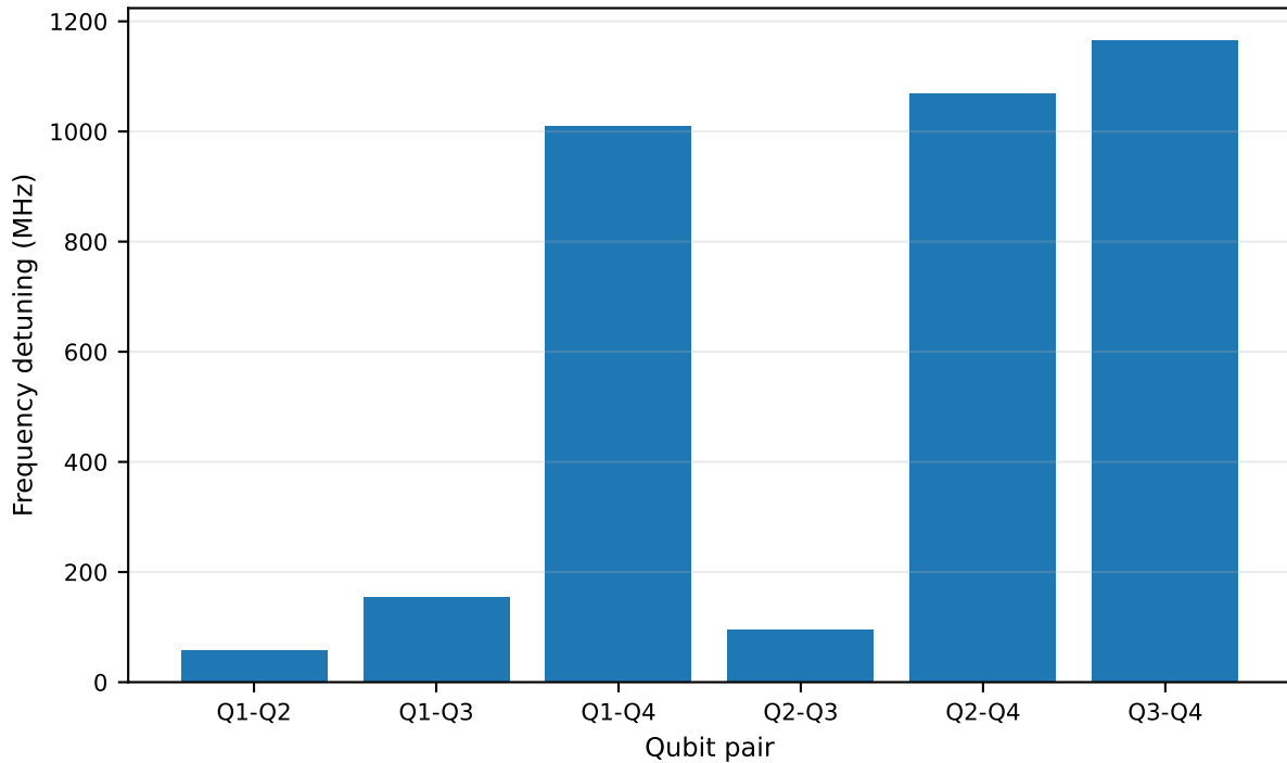
Provisional qubit-pair frequency detunings
