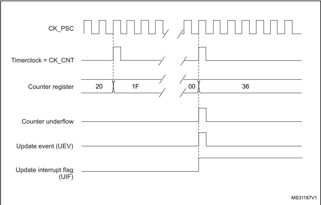
Figure 106. Counter timing diagram, Update event when repetition counter is not used
