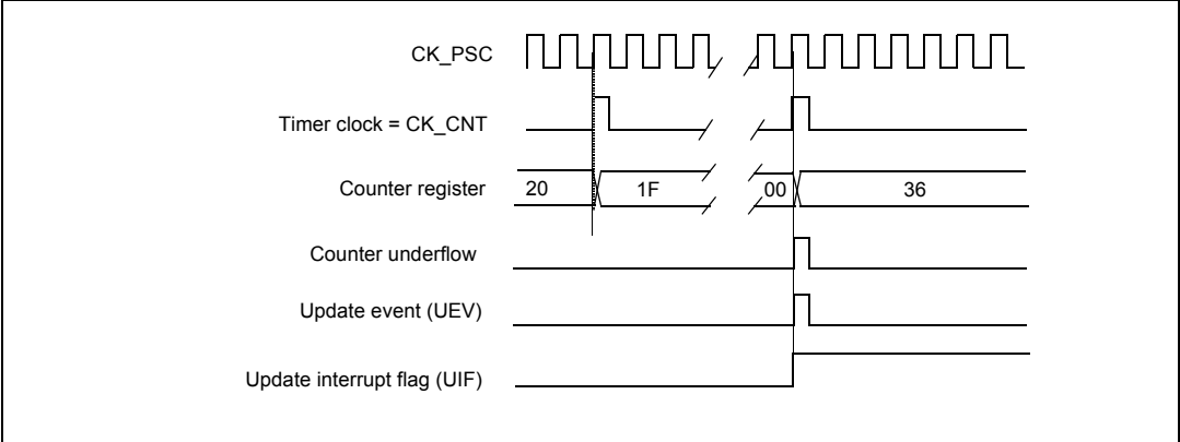
Figure 57. Counter timing diagram, internal clock divided by N
