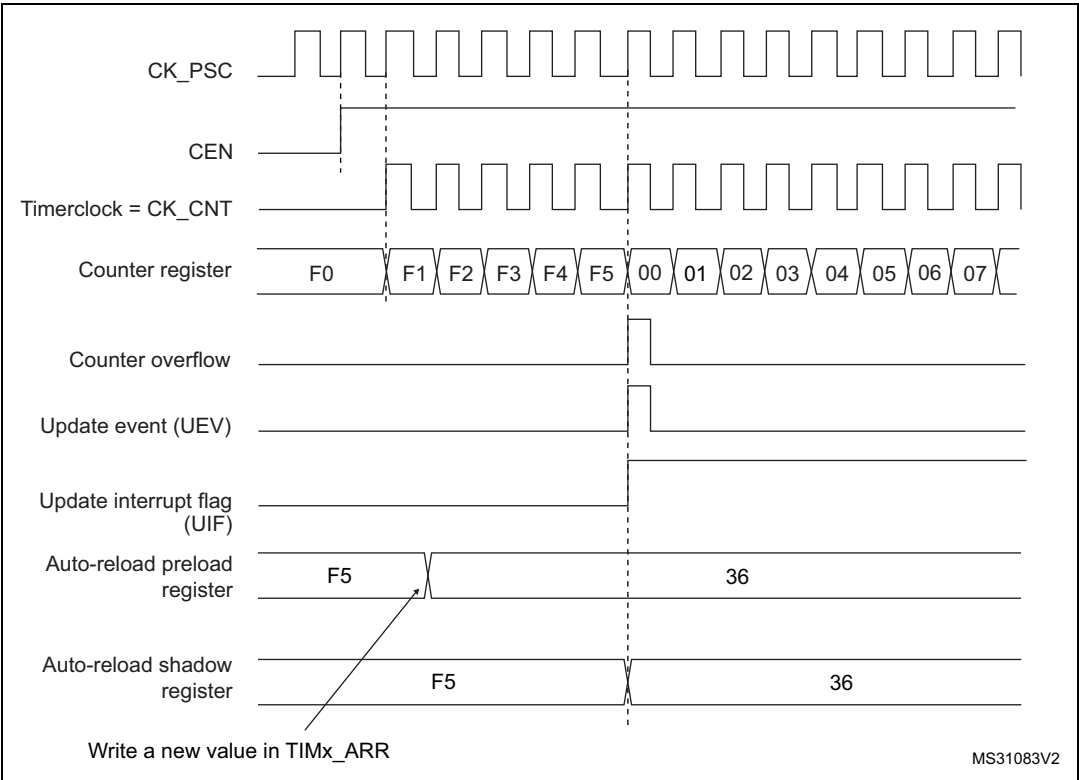
Figure 147. Counter timing diagram, update event when ARPE=1 (TIMx_ARR preloaded)
