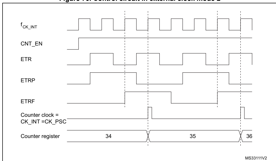
Figure 70. Control circuit in external clock mode 2
