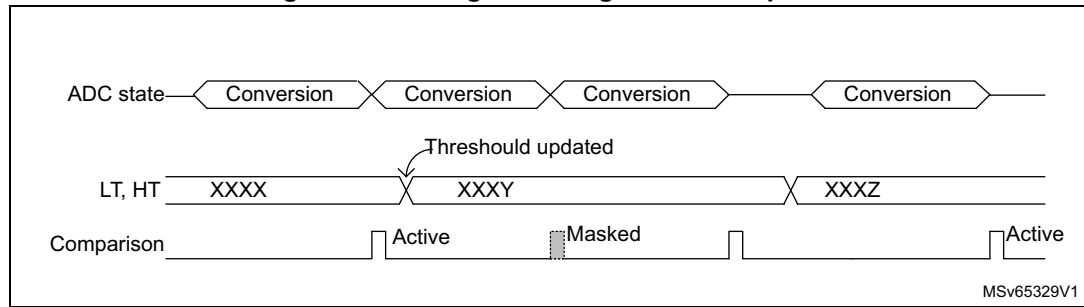
Figure 43. Analog watchdog threshold update
