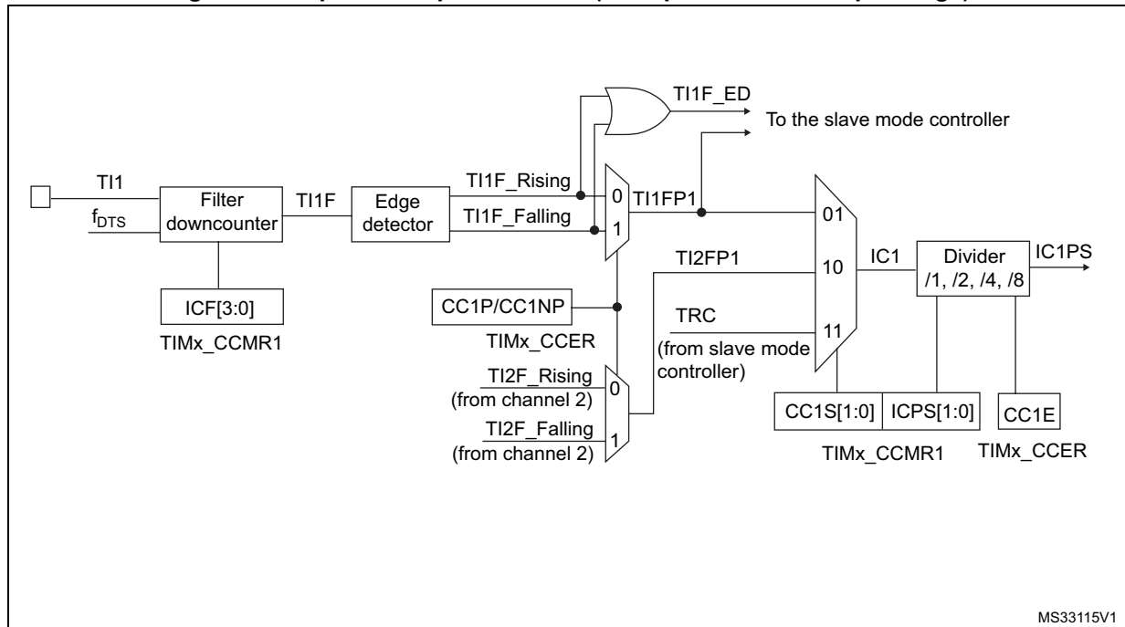
Figure 71. Capture/compare channel (example: channel 1 input stage)
