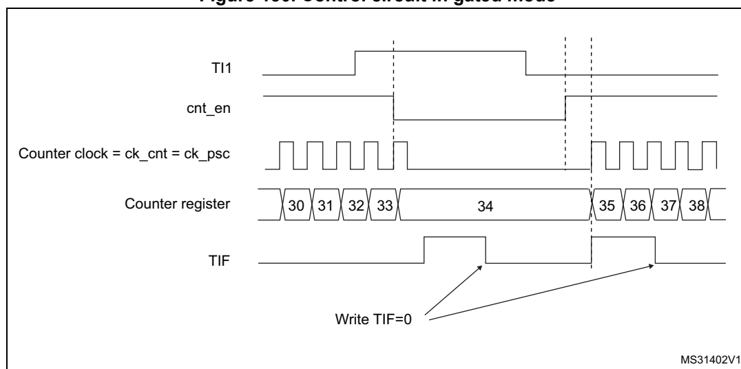
Figure 130. Control circuit in gated mode
