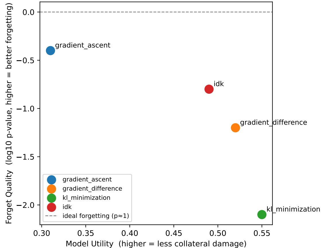
TOFU: Forget Quality vs Model Utility
