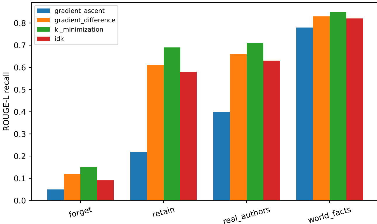
ROUGE by split (left = should drop, right = should stay high)
