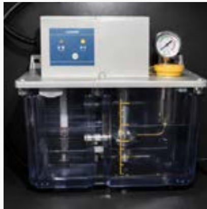
Lubrication system "BAOTENG" Oil lubricant Made in China
