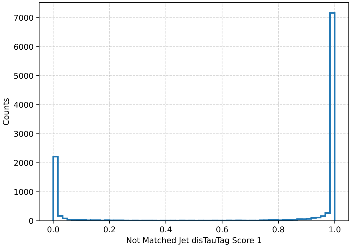
Stau_100_100mm Jet disTauTag Score 1
