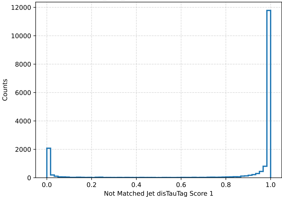
Stau_100_10mm Jet disTauTag Score 1
