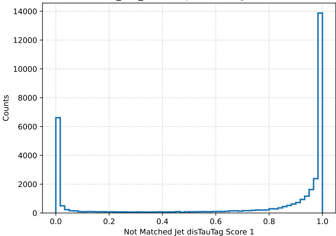
Stau_200_1000mm Jet disTauTag Score 1
