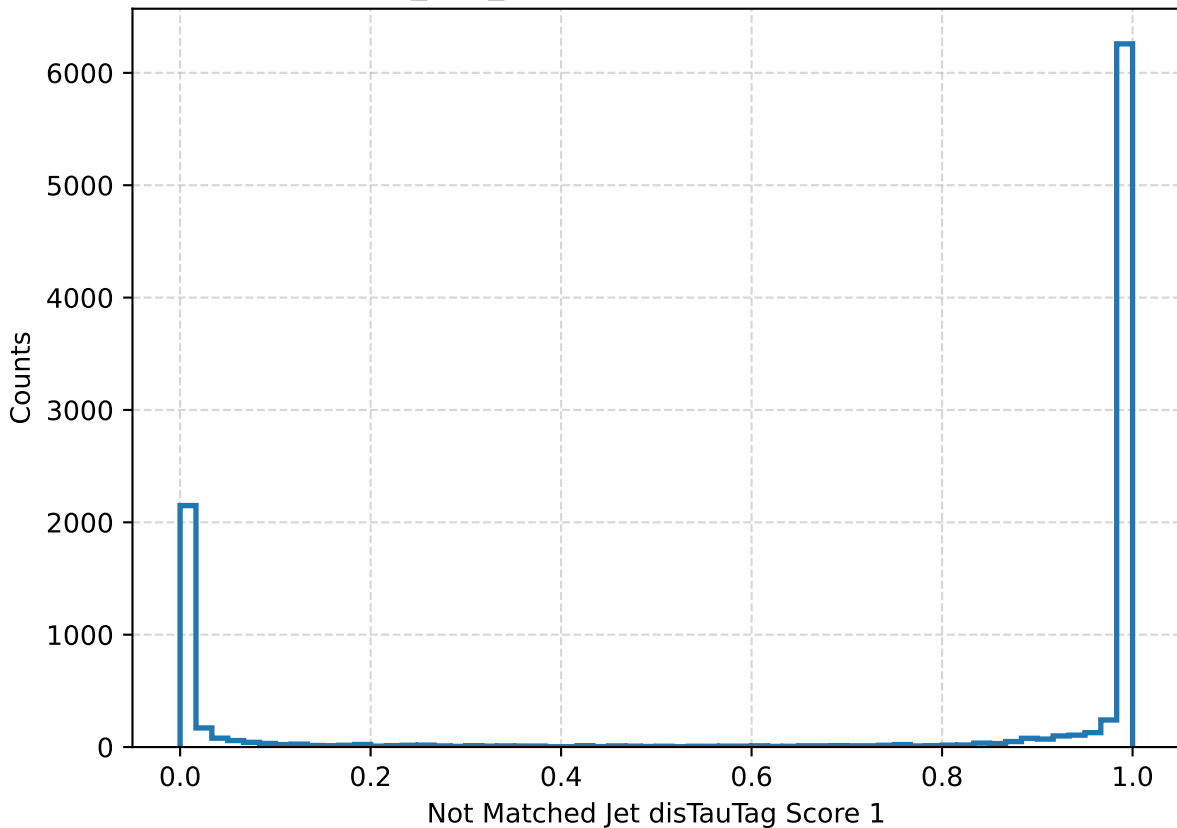
Stau_200_100mm Jet disTauTag Score 1
