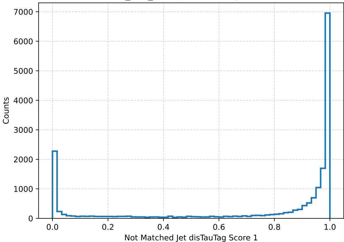
Stau_200_1mm Jet disTauTag Score 1
