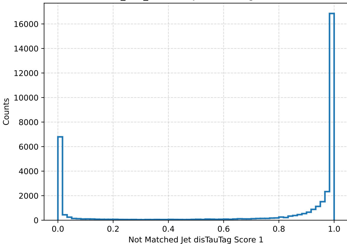
Stau_300_1000mm Jet disTauTag Score 1
