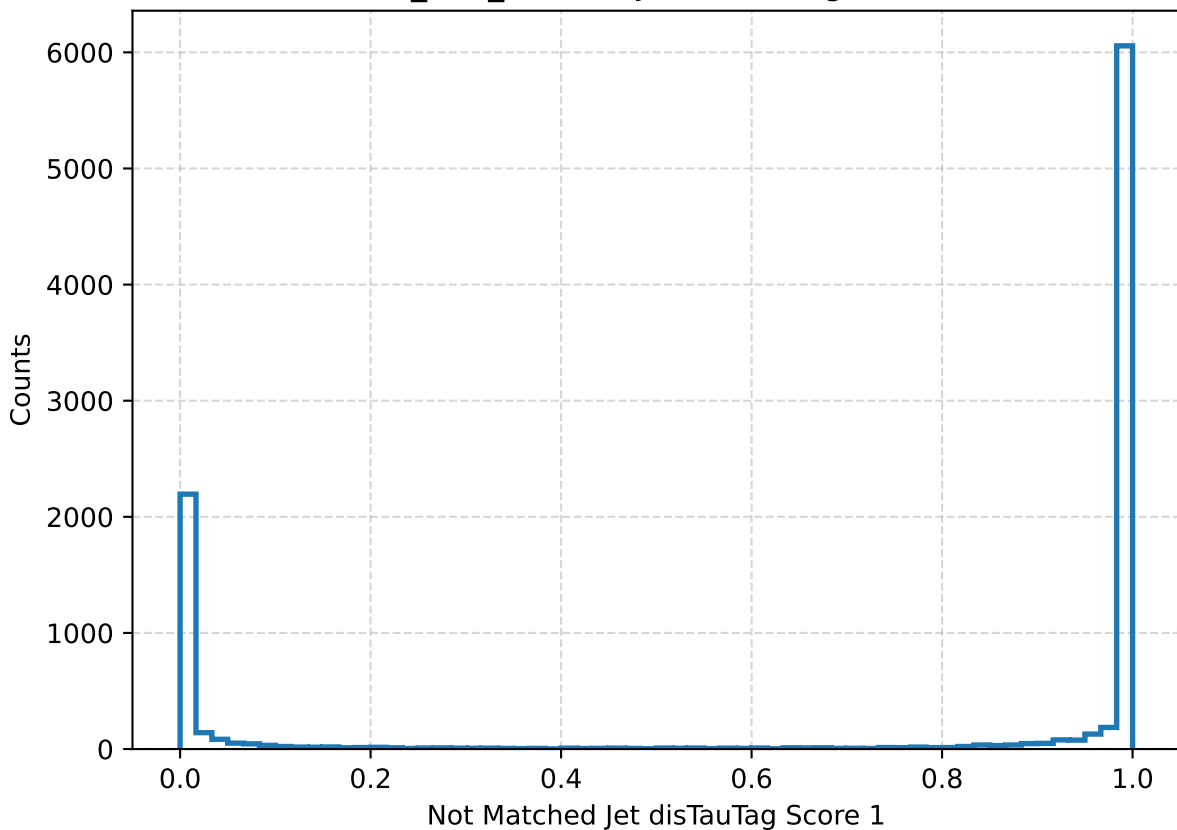
Stau_300_100mm Jet disTauTag Score 1
