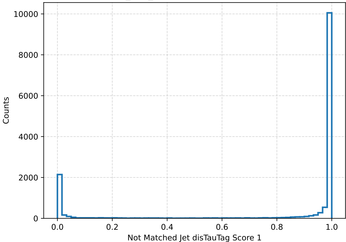
Stau_300_10mm Jet disTauTag Score 1
