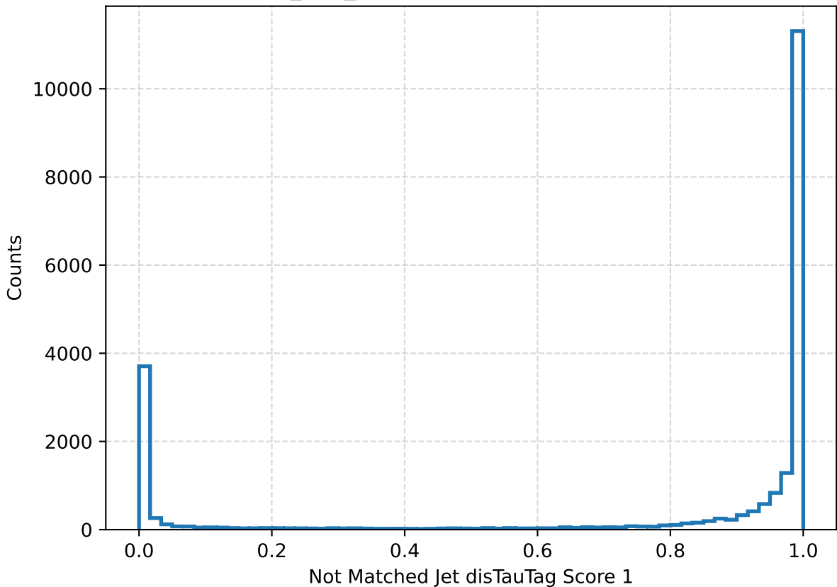
Stau_500_1000mm Jet disTauTag Score 1
