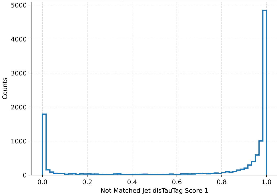
Stau_500_1mm Jet disTauTag Score 1
