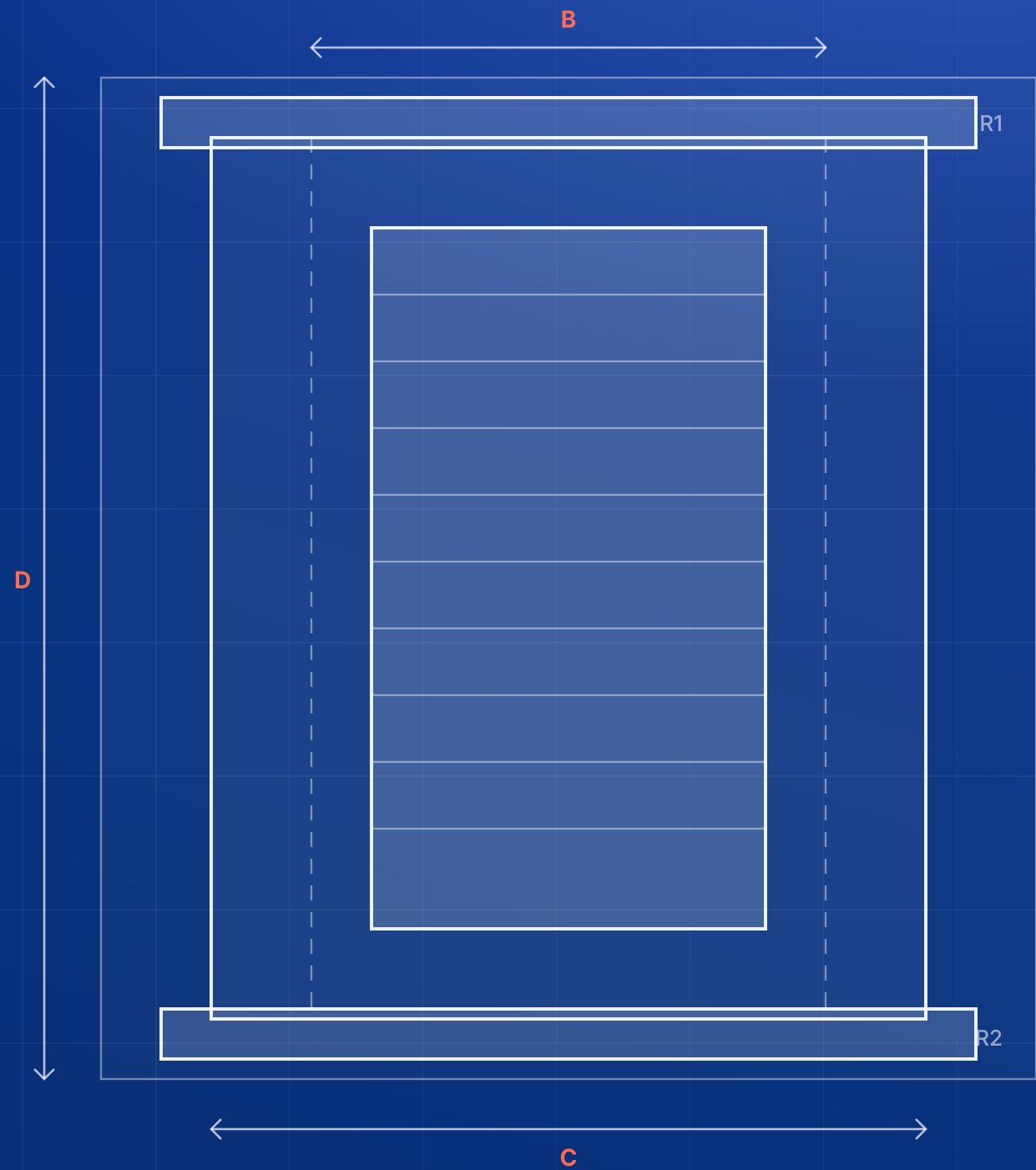
B HANDRAIL CENTRES · C TRUSS WIDTH · D CLEAR WELL LENGTH
