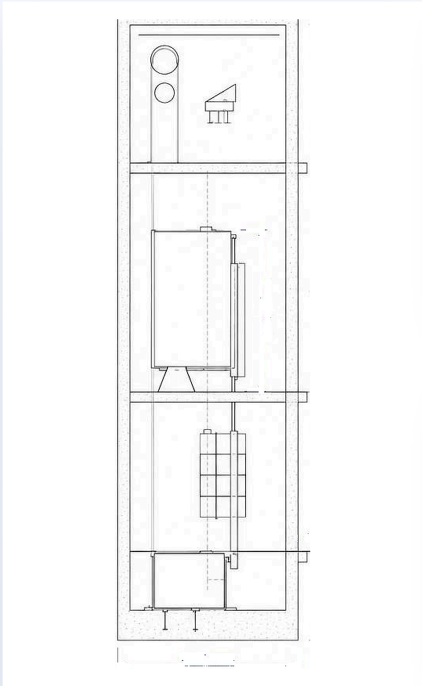
ELEVATOR SHAFT · SECTION
