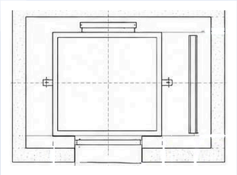
SHAFT LAYOUT · PLAN
