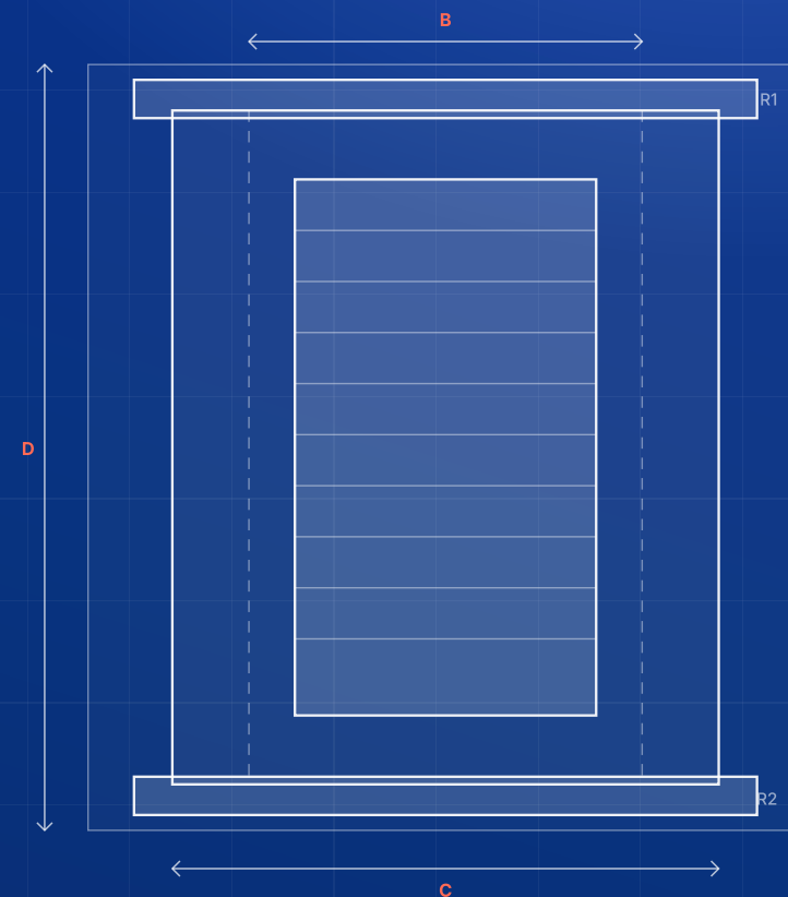
B HANDRAIL CENTRES · C TRUSS WIDTH · D CLEAR WELL LENGTH
