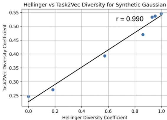
Figure 6: Task2Vec diversity coefficient correlates with ground truth diversity for synthetic Gaussian benchmark. Source: (Miranda et al., 2022b)
