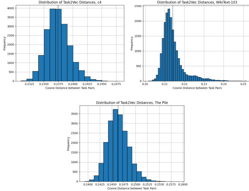
Figure 9: Distributions of pairwise batch distances from C4 (top left), WikiText-103 (top right), and The Pile (bottom) are approximately Gaussian, which justifies the use of a sample of batches to measure the diversity coefficient. Dotted lines indicate the average distance, i.e. the diversity coefficient, for each dataset.
