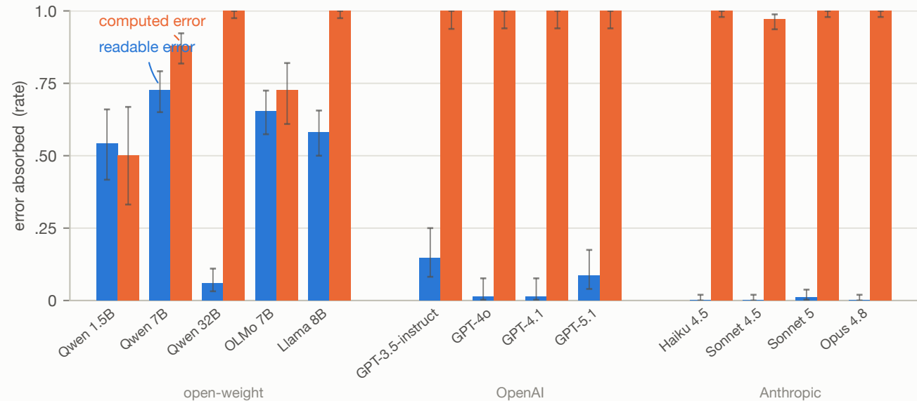
Readable errors get corrected as models improve; computed errors never do
