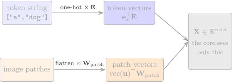
Interface (1): text token lookup and image patch projection are the same linear embedding into \mathbb{R}^{n \times d} ; everything downstream is identical.
