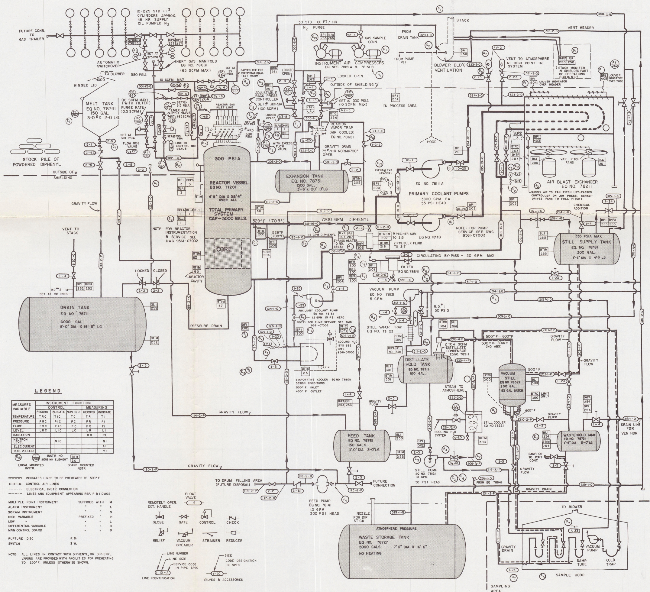
Fig. 9. Piping and Instrumentation Diagram
