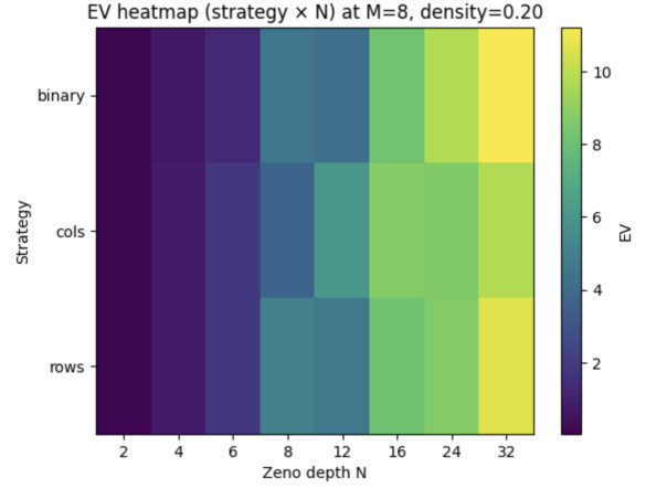
(b) Strategy \times N heatmap. EV of all 3 strategies compared with increasing Zeno depth.
