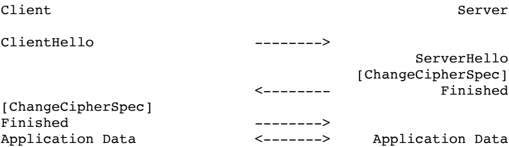
Figure 2. Message flow for an abbreviated handshake
