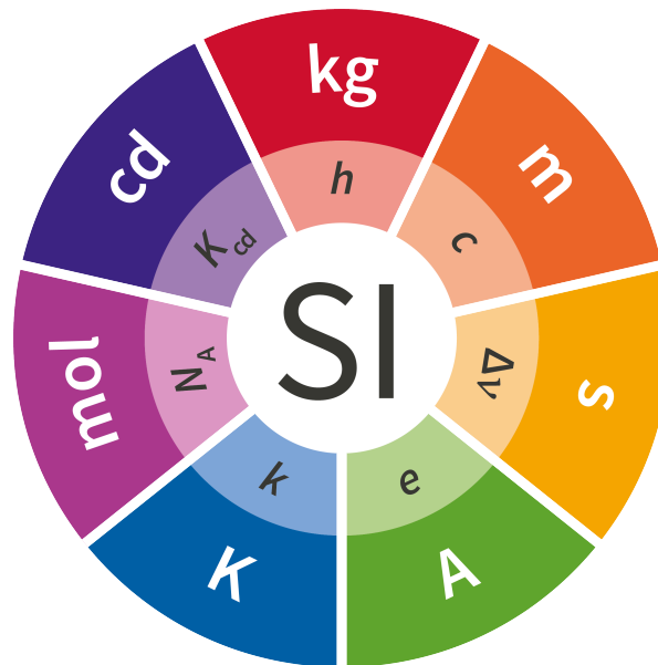
Figure 1: Defining the International System of Units (SI).
