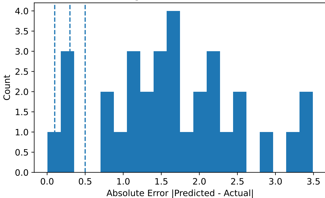
Histogram of Absolute Error
