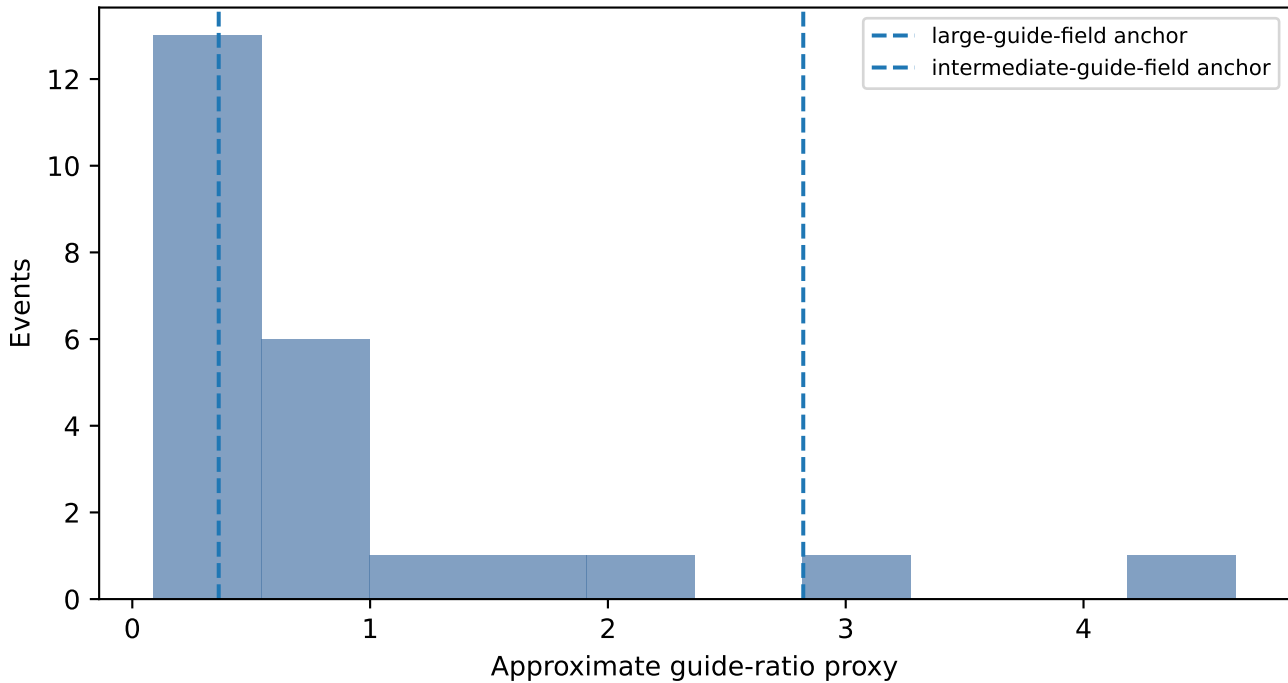
Guide-field proxy (not ground truth)
