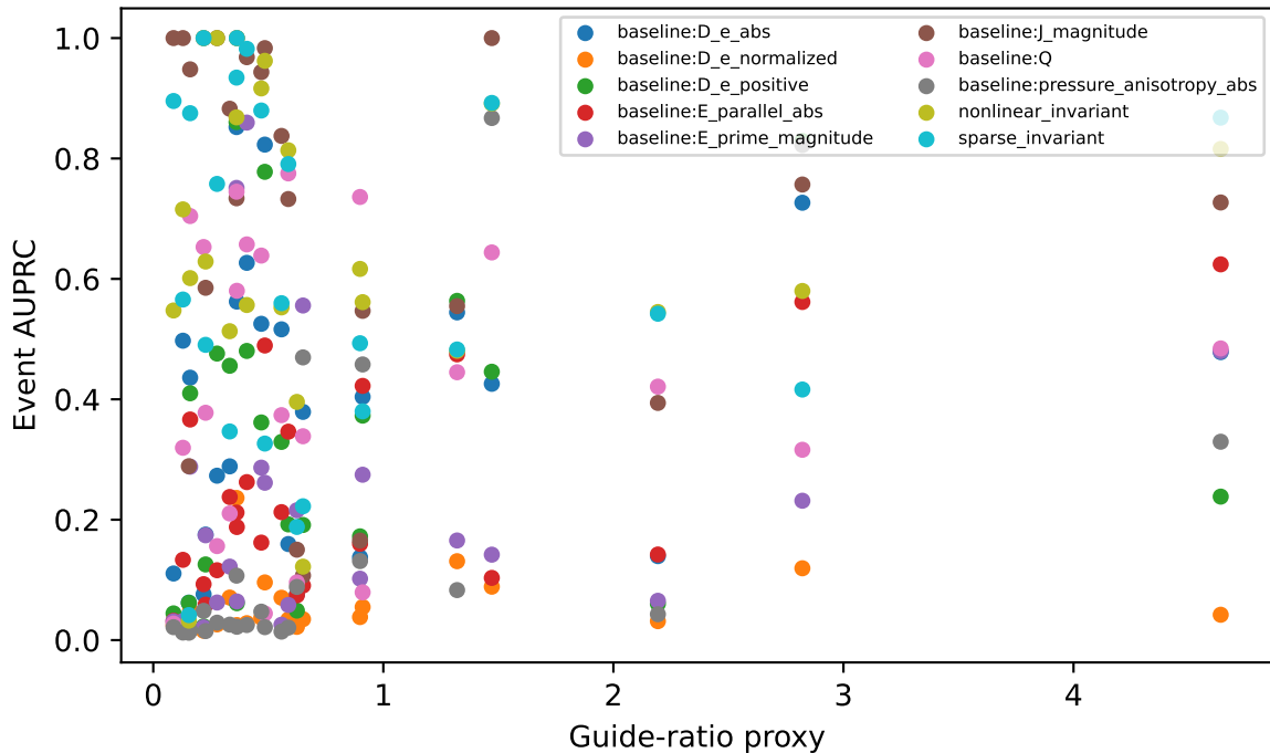
Performance versus approximate guide field
