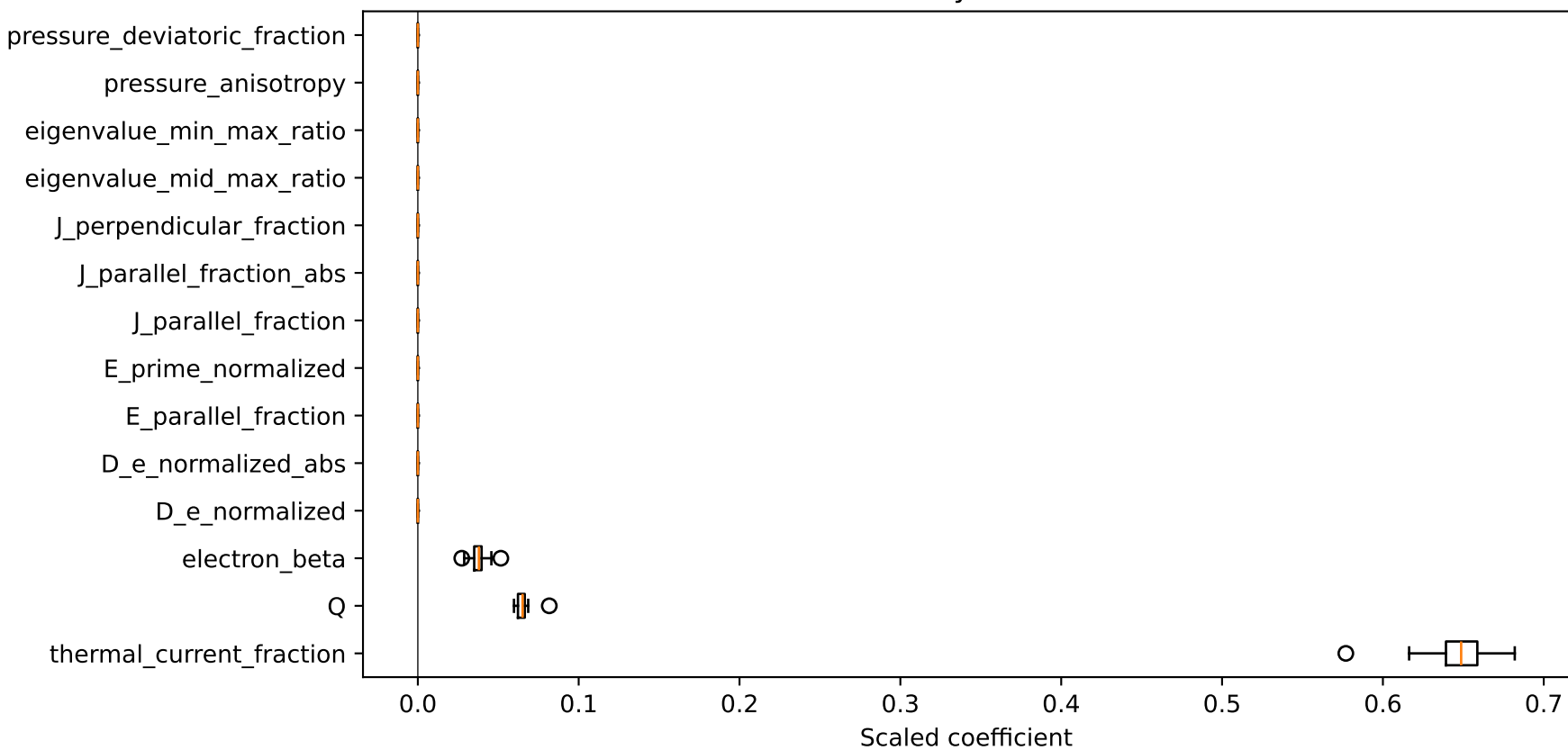
L1 coefficient stability across held-out folds
