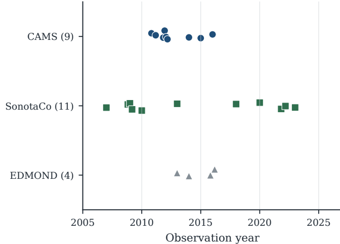
D External matches by year
