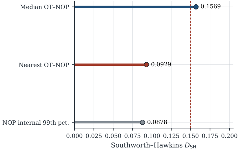
C Orbital separation
