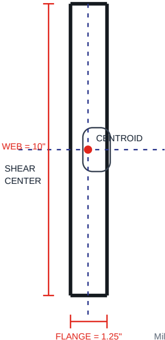
CAD SECTION
