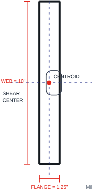
CAD SECTION
