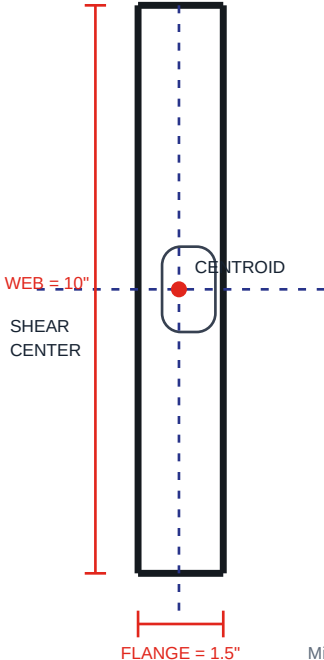
CAD SECTION
