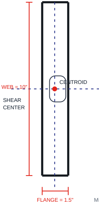
CAD SECTION
