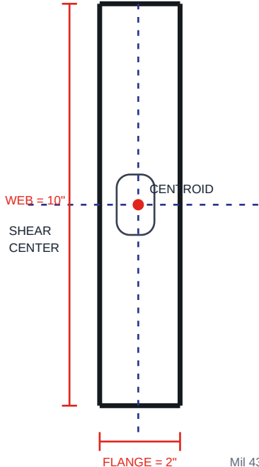
CAD SECTION
